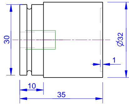
Knob Aluminium
