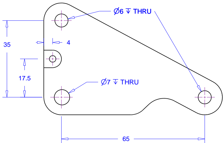
Moving Jaw
