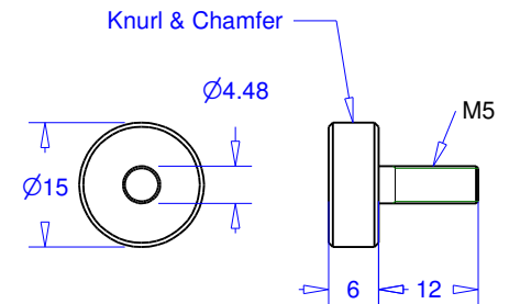
Stop Bar Clamp Screw (1off Brass)
