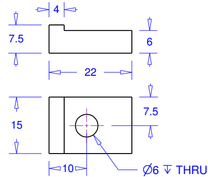
Clamp Plate (1off M.S.)
