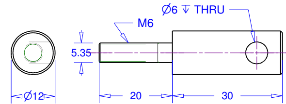
Clamp Screw (1off M.S.)
