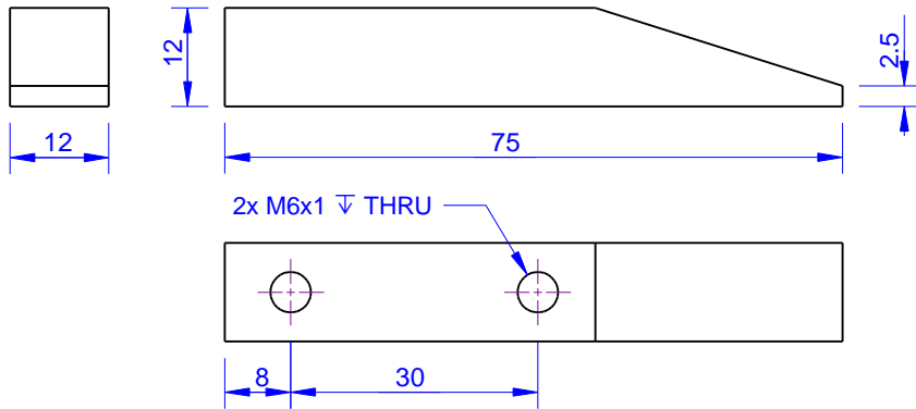
Moving Jaw
