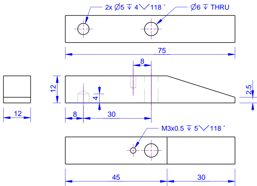
Fixed Jaw
